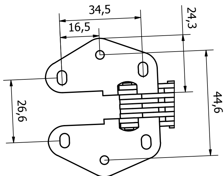
VIEW B ( 1 : 1 )
